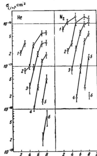
FIG. 2. Dependence of \sigma_{i,i+1} on the atomic number Z for v = 8 \times 10^8 cm/sec in helium and nitrogen. The initial ionic charge i is marked near the curves.
