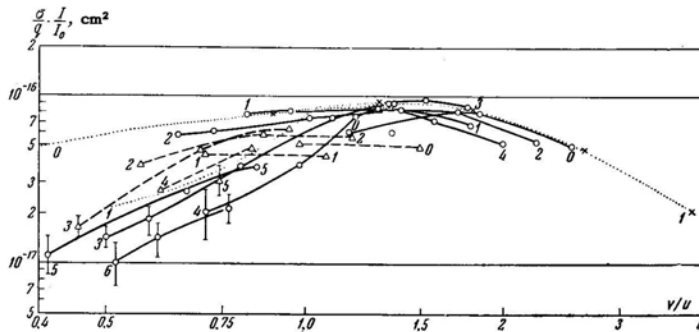
FIG. 8. Dependence of \sigma_{i, i+1}/qI_0 on v/u for He ( \times ), N ( \circ ) and Ne ( \Delta ) ions in helium ( I_0 = 13.5 eV). The values of i are marked by the curves. The values of \sigma_{0,1} for helium atoms were taken from Allison's review. [1]
