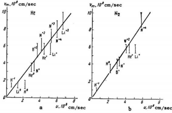
FIG. 5. Relationship between the velocities u and v_m for various ions in helium and nitrogen.
