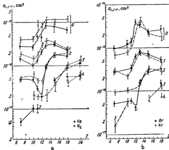
FIG. 3. Dependence of \sigma_{i,i+1} on Z for v = 2.6 \times 10^8 cm/sec in helium, nitrogen, argon, and krypton. The initial ionic charge i is marked near the curves.
