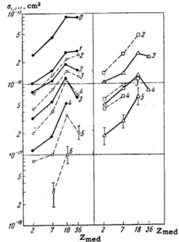
FIG. 4. Dependence of \sigma_{i,i+1} on the atomic number of atoms in the gaseous medium, Z_{\text{med}} , for Ne ions ( v = 4.1 \times 10^8 cm/sec, denoted by black dots, and v = 5.6 \times 10^8 cm/sec, denoted by open circles), P ions (denoted by \square ) and Ar ions ( v = 4.1 \times 10^8 cm/sec, denoted by \Delta ).
