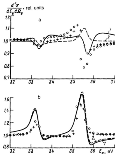
FIG. 4. Spectrum of electrons ejected at an angle of 16^\circ (a) and 60^\circ (b): result of the ionization of helium atoms by 100-keV protons: 1) calculation allowing for the dependence of K_{res,\mu} on the electron energy; 2) calculation in the E_e = E_\mu approximation for the K_{res,\mu} factor. In both calculations a convolution is formed with the Gaussian distribution characterized by an average energy scatter of 0.13 eV. Experimental points: + ) Ref. 27; o) Ref. 26.
