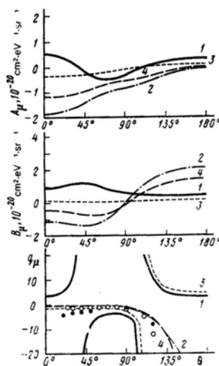
FIG. 2. Angular dependences of the asymmetry parameter A_\mu(E_i, \theta_e) , of the yield parameter B_\mu(E_i, \theta_e) , and of the profile index \bar{q}_\mu(E_i, \theta_e) of a (2s^2)^1S resonance in the spectrum of electrons emitted as a result of ionization of helium atoms by protons: 1), 3) calculation in the approximation based on E_i = E_\mu for the K_{res,\mu} factor; 2), 4) calculation in the Born approximation for energies 300 and 500 keV, respectively; experimental data from Ref. 28: (●) 300 KeV; (○) 500 keV.
