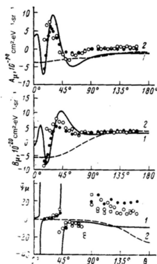
FIG. 1. Angular dependences of the asymmetry parameter A_\mu(E_i, \theta_e) , of the yield parameter B_\mu(E_i, \theta_e) , and of the profile index \bar{q}_\mu(E_i, \theta_e) of a (2s^2)^1S resonance in the spectrum of electrons ejected as a result of ionization of helium atoms by 100-keV protons: 1) calculation in the E_i = E_\mu approximation for the factor K_{res,\mu} ; 2) calculation in the Born approximation. Experimental points: (●) Ref. 27; (○) Ref. 28.
