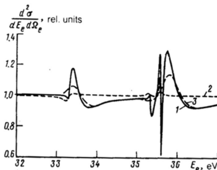
FIG. 3. Spectrum of electrons ejected at an angle of 0^\circ as a result of ionization of helium atoms by 100-keV protons: 1) calculated allowing for the dependence of K_{res,\mu} on the electron energy; 2) calculation in the E_e = E_\mu approximation for the K_{res,\mu} factor; 3) convolution of a calculated spectrum 1 with a Gaussian distribution characterized by an average energy scatter of 0.13 eV.
