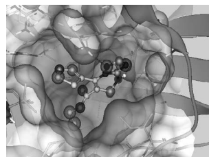
The location of compound 5 in the pocket of DHFR
