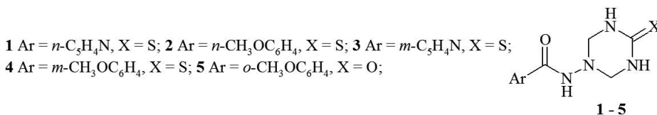
Fig. 1. Structural formulas of modeled compounds.
