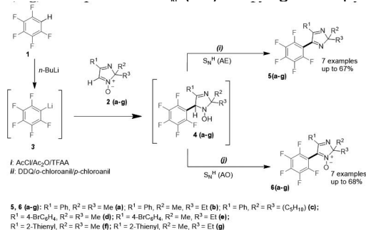
Scheme 1. Coupling of pentafluorophenyl lithium with 2H-imidazole-1-oxide
