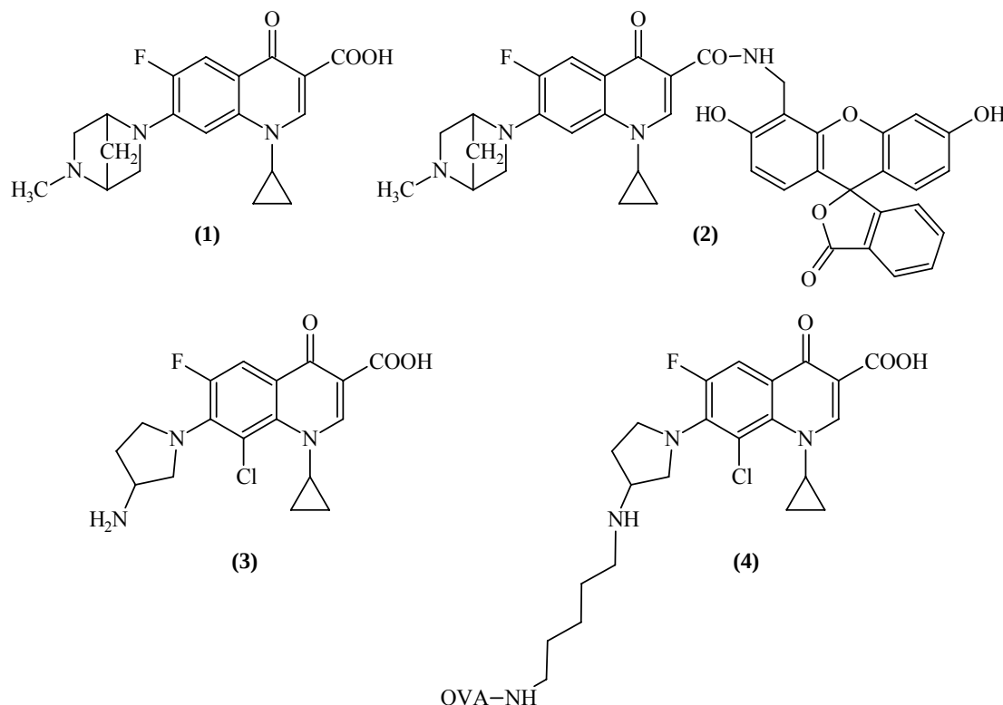
Fig. 1: Structure of main analytes and conjugates used in the study: danofloxacin (1), DAN-4AMF tracer (2), cinafloxacin (3), and CLI-NH-C5-NH-OVA conjugate (4)
